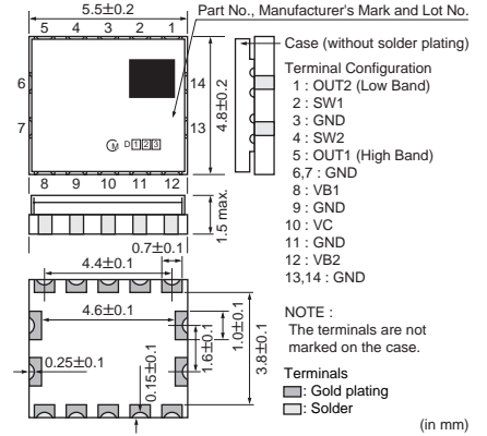
MQW5 SERIES
