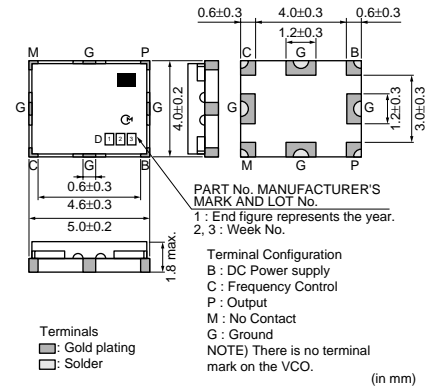
MQL SERIES
