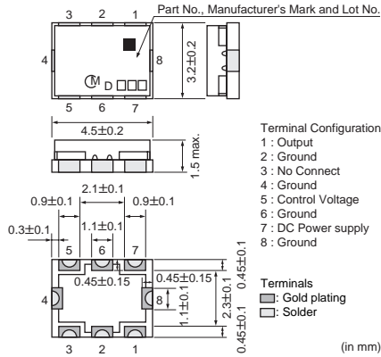
MQR SERIES
