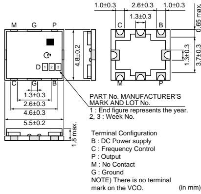
MQK SERIES
